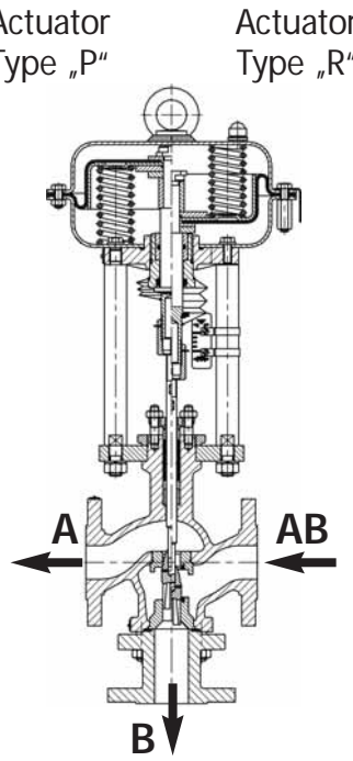
Fig. 4 P/R-BR 13 Diverting service
