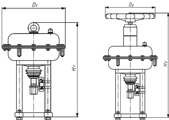
Fig. 6: actuators type P/R, PN/RN
