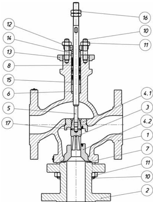
Fig. 1 Control valve
